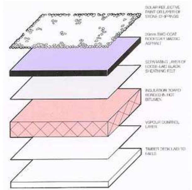
Fig. 1.26 WARM ROOF
